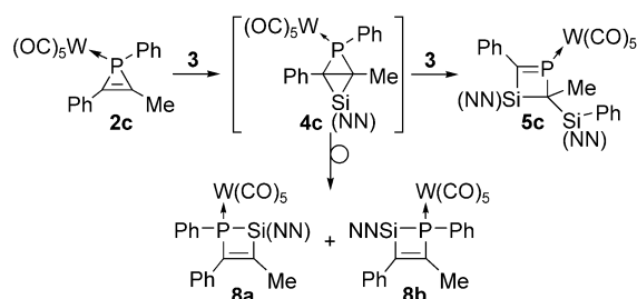
Scheme 3. Isomerization of 4c .
